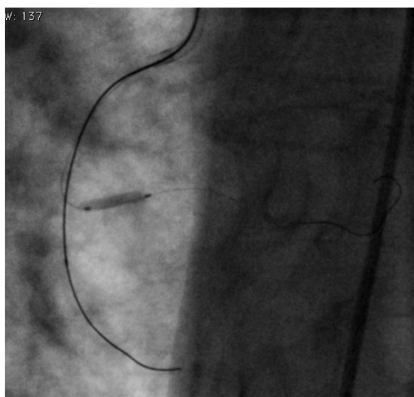
Figure 2. Ultimate Bros 3 wire across the lesion and marker of the Tornus system, creating space in the occlusion. Anchor technique (BMW Universal II with 2.5 mm x 15 mm Maverick MONORAIL balloon catheter in the right coronary branch)
